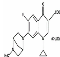
Chemical structure of Danofloxacin Mesylate
