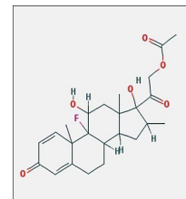
Chemical structure of Dexamethasone acetate
