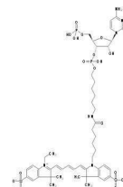
Chemical structure of pCp-CY5 (Cy5)
