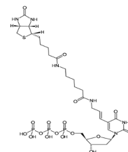
Chemical structure of Biotin-11-dUTP (Biotin).
