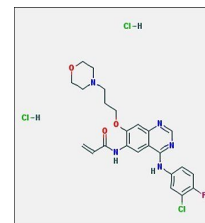
Chemical structure of Canertinib, Dihydrochloride Salt
