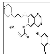
Canertinib, Dihydrochloride Salt: Cl-1033, Canertinib HCl
