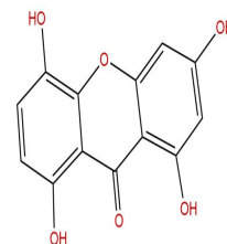
1,3,5,8-Tetrahydroxyxanthone
