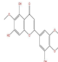
Chemical structure of 5,7,3'-Trihydroxy-6,4',5'-trimethoxyflavone
