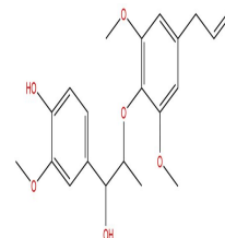
1-(3,4-dimethoxyphenyl)-2-(4-allyl-2,6-dimethoxyphenoxy)propan-1-ol
