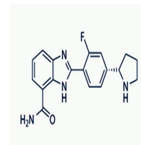
Chemical structure of A-966492
