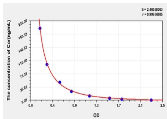
Standard curve for orb782688 ELISA kit.
