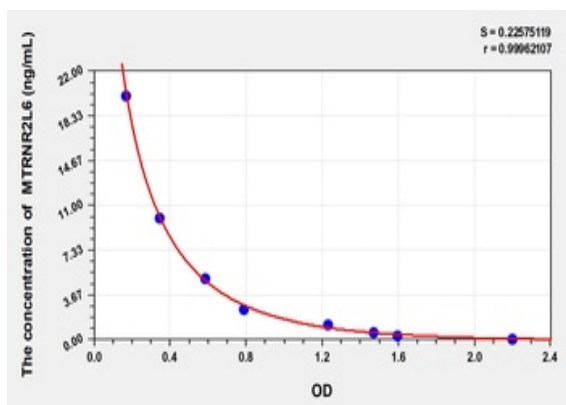
Standard curve for orb782561 ELISA kit.
