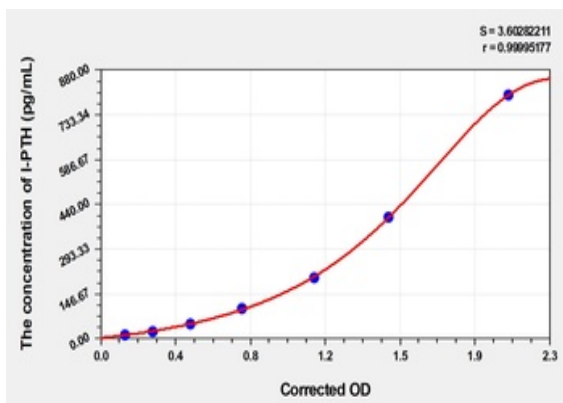
Standard curve for orb781647 ELISA kit.
