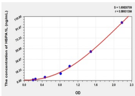
Standard curve for orb781601 ELISA kit.
