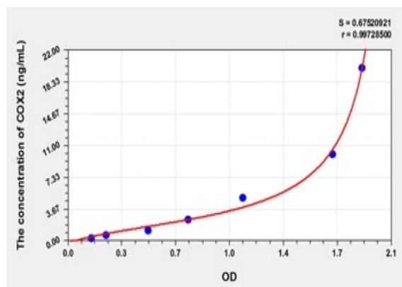
Standard curve for orb781472 ELISA kit.
