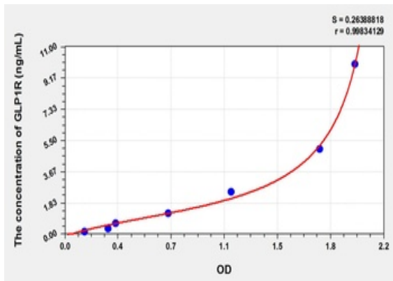
Standard curve for orb781428 ELISA kit.
