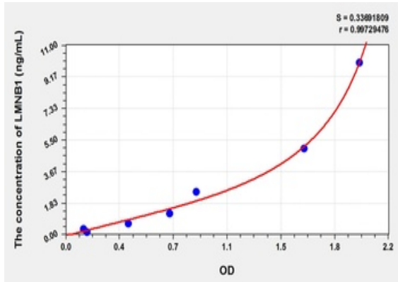
Standard curve for orb781279 ELISA kit.
