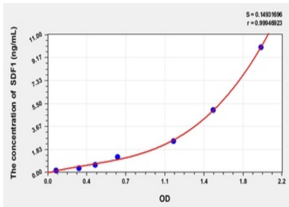
Standard curve for orb781069 ELISA kit.
