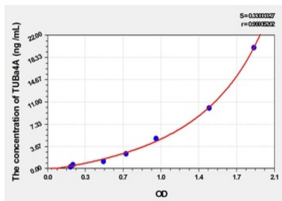
Standard curve for orb780652 ELISA kit.
