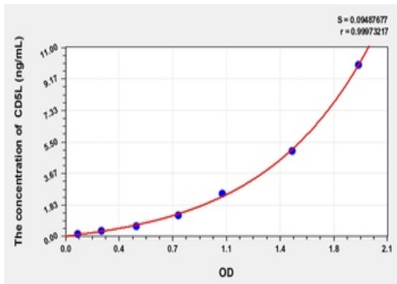
Standard curve for orb780648 ELISA kit.
