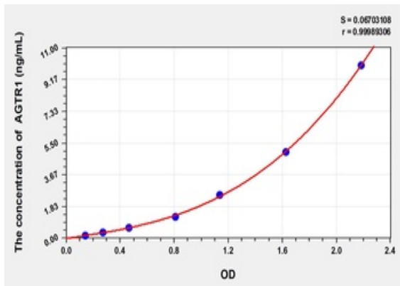
Standard curve for orb780482 ELISA kit.
