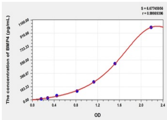
Standard curve for orb779805 ELISA kit.
