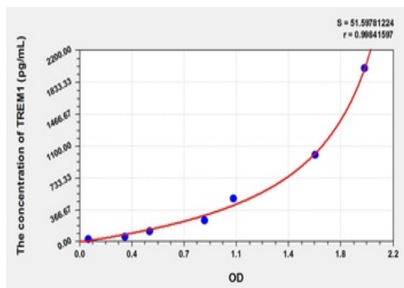
Standard curve for orb779681 ELISA kit.
