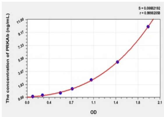
Standard curve for orb779511 ELISA kit.
