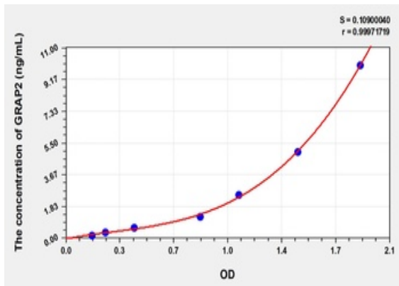
Standard curve for orb779056 ELISA kit.
