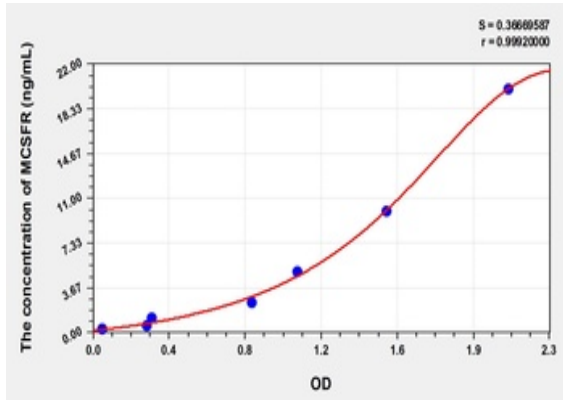
Standard curve for orb779047 ELISA kit.
