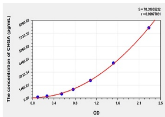
Standard curve for orb779030 ELISA kit.
