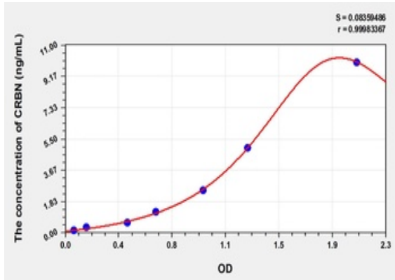
Standard curve for orb778732 ELISA kit.
