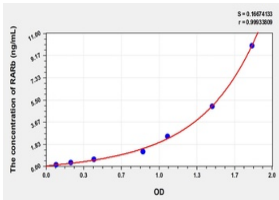
Standard curve for orb778300 ELISA kit.
