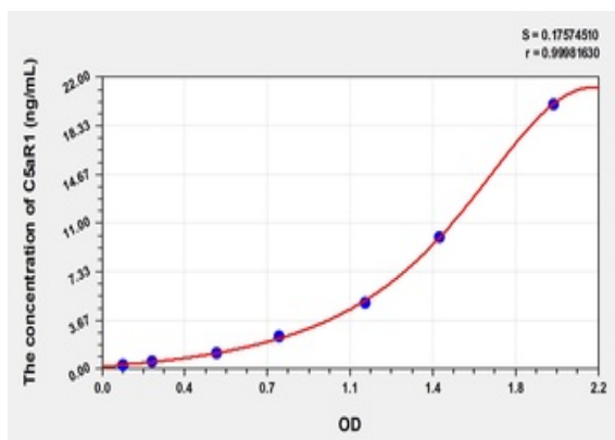
Standard curve for orb778107 ELISA kit.
