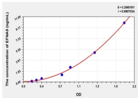
Standard curve for orb777963 ELISA kit.
