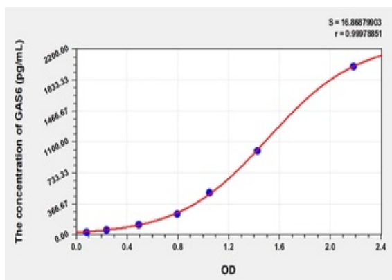
Standard curve for orb777746 ELISA kit.
