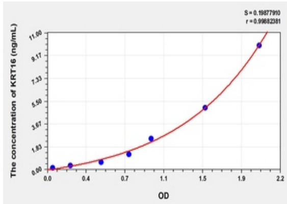
Standard curve for orb777731 ELISA kit.
