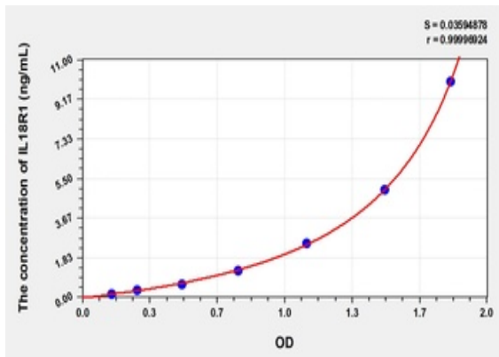
Standard curve for orb777336 ELISA kit.
