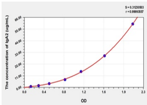
Standard curve for orb777313 ELISA kit.
