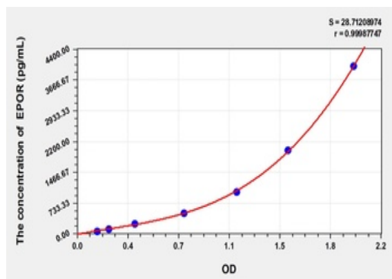
Standard curve for orb776345 ELISA kit.
