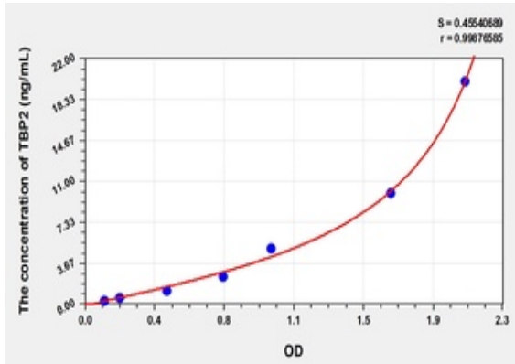
Standard curve for orb776323 ELISA kit.
