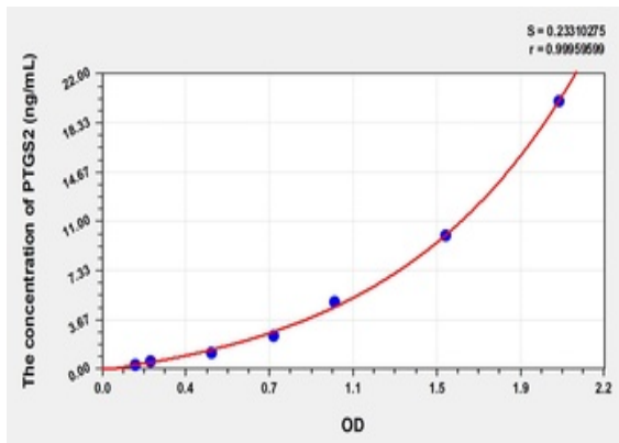
Standard curve for orb775960 ELISA kit.
