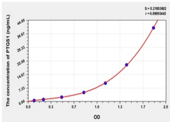
Standard curve for orb775722 ELISA kit.
