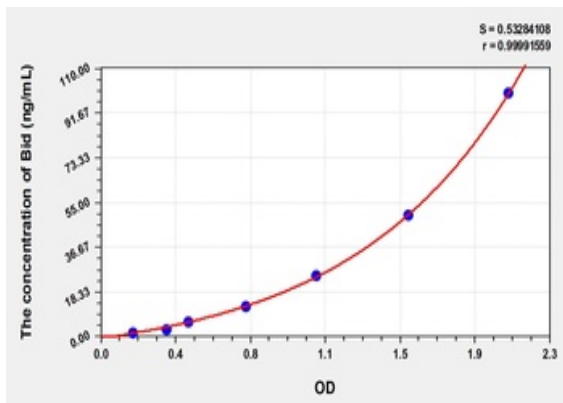
Standard curve for orb775567 ELISA kit.
