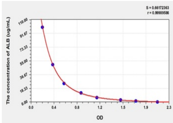
Standard curve for orb775246 ELISA kit.
