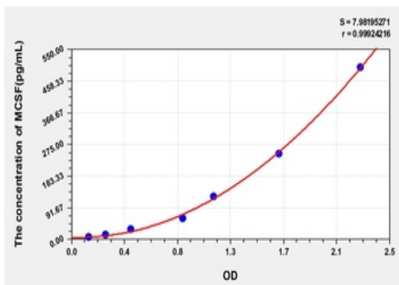
Standard curve for orb775033 ELISA kit.
