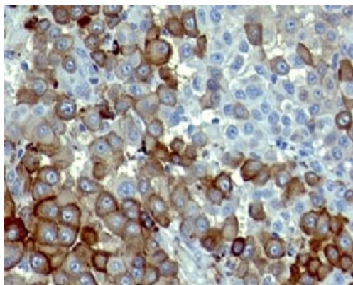
IHC: Formalin-fixed, paraffin-embedded human melanoma stained with NGFR antibody (NTR/912).
