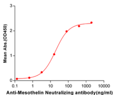
Anti-Mesothelin (amatuximab biosimilar) mAb ELISA 0.2 µg of Mesothelin(296-580), mFc-His Tagged protein per well
