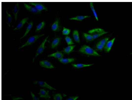
Immunofluorescence analysis of Hela Cells using CYP17A1 antibody
