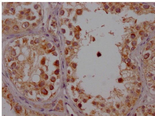
Immunohistochemical staining of human testis tissue using CYP17A1 antibody
