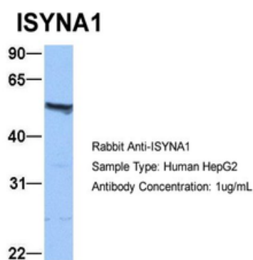
Sample Type: HepG2, Antibody dilution: 1.0 ug/ml. ISYNA1 is supported by BioGPS gene expression data to be expressed in HepG2.
