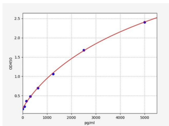
Standard curve for orb566908 ELISA kit.
