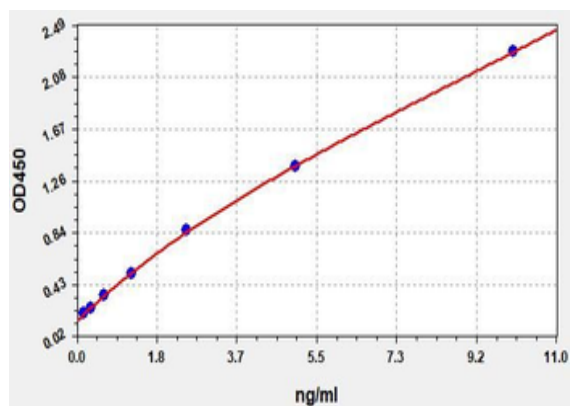
Standard curve for orb565800 ELISA kit.
