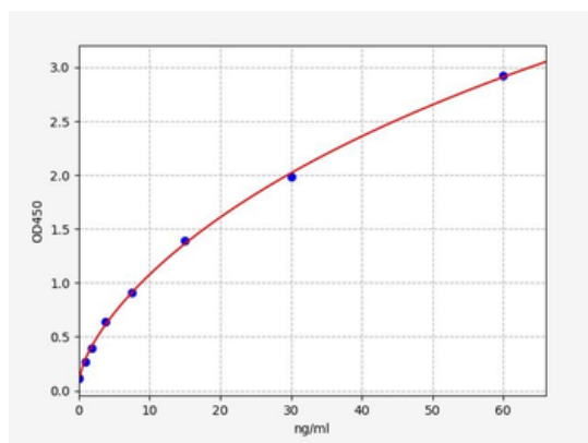
Standard curve for orb565352 ELISA kit.
