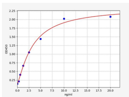
Standard curve for orb563977 ELISA kit.
