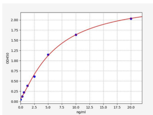
Standard curve for orb563636 ELISA kit.
